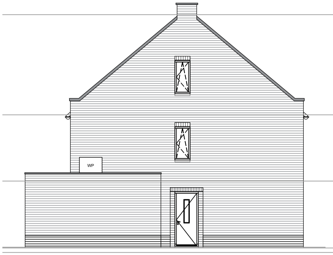
Linkergevel kavel 10, 12
