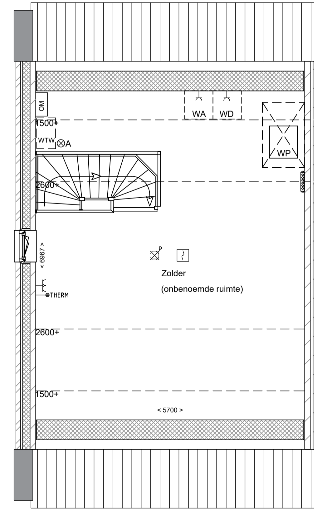
Zolder 10, 12
